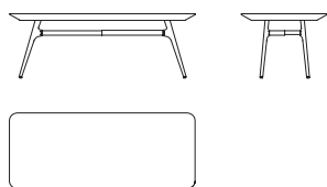
RT009-12_SPAZIOXL22 220x100 cm | H 78 cm
